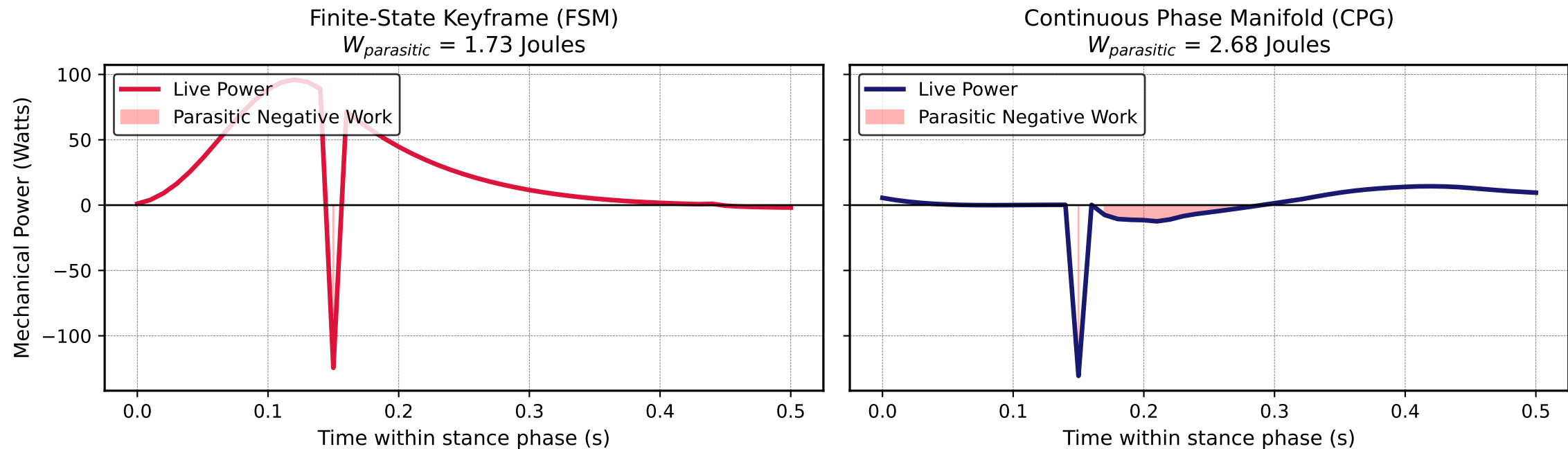
Fig. 3. Instantaneous mechanical power dissipation at the trailing ankle joint during late stance. Shaded regions denote parasitic negative work ( W_{parasitic} ) caused by the rigid spatial tracking of static dictionary keyframes.
